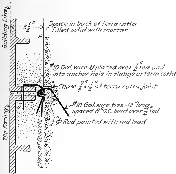
METHOD OF ANCHORING TERRA COTTA TO CONCRETE COLUMNS
